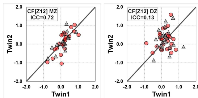
FIGURE 7. Correlation of the Z12 CF between twin pairs. SA CF for twins 1# plotted against twins 2# for MZ ( left graph ) and DZ ( right graph ) twin pairs. Circles and triangles represent right and left eyes. The solid line represents the Y = X identity. ICCs are shown in each graph.
