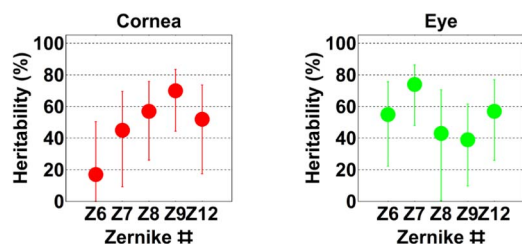
FIGURE 4. Heritability of optical aberrations. Heritability of several aberration coefficients (Z6 and Z9 are trefoils, Z7 and Z8 are comas, and Z12 is SA) of the cornea ( left graph ) and the total eye ( right graph ). Error bars represent the 95% confidence intervals for the estimation of heritability.
