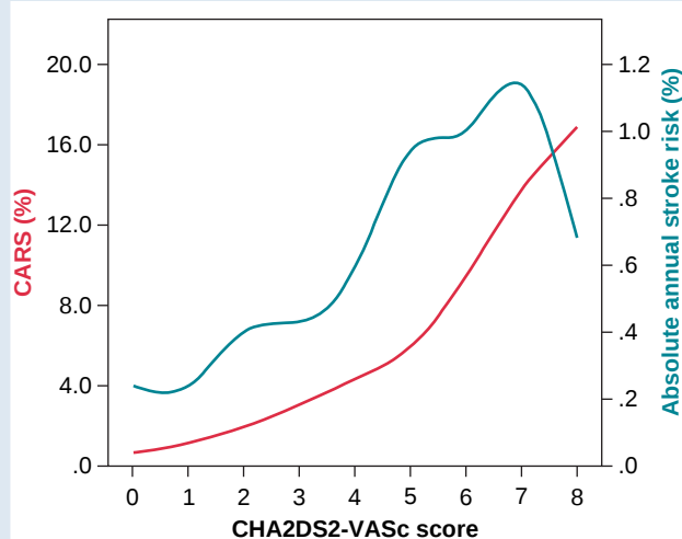
Figure 2 Plot of CARS vs. absolute annual stroke risk stratified by CHA 2 DS 2 -VASc score.
