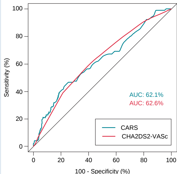
Figure 1 Receiver-operating characteristic curves for absolute stroke events by CARS vs. CHA 2 DS 2 -VASc score.
